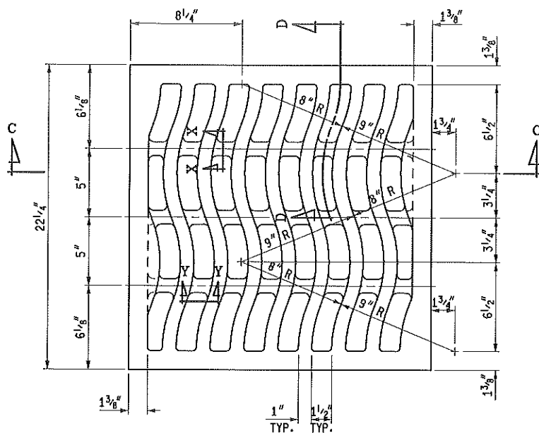
PLAN VIEW OF GRATE
