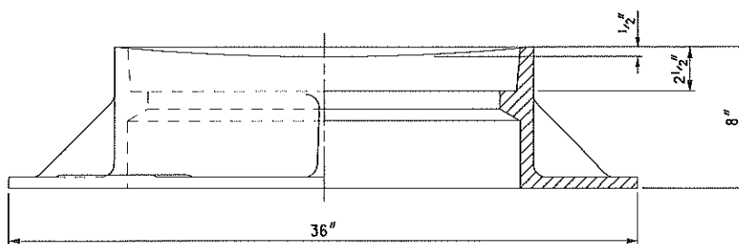
HALF SIDE ELEVATION
